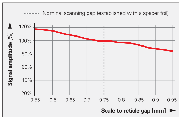
Influence of the scanning gap on the signal amplitude for ERA 4000
