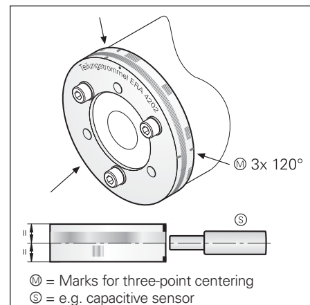
Three-point centering
