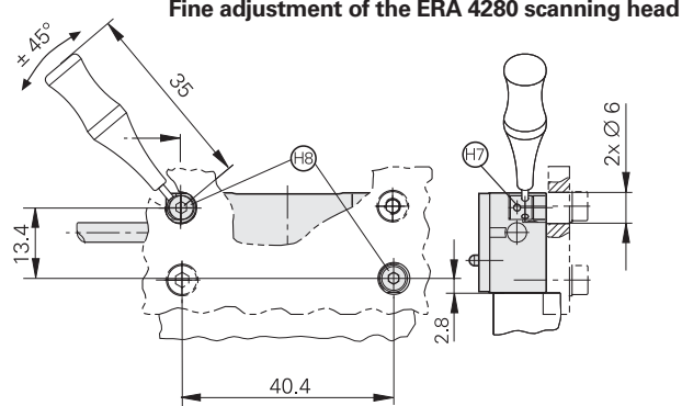
Fine adjustment of the ERA 4280 scanning head
